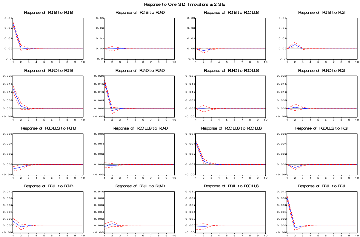
Figure 1. Impulse response functions of the variables to a one standard deviation shock.
